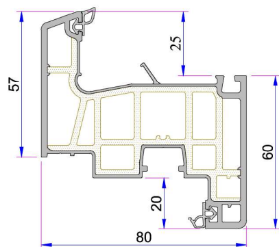
Sash Profile P.A.883.2000.600.2.BC.01
