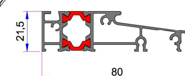
Alm. Threshold Profile (In Process)
