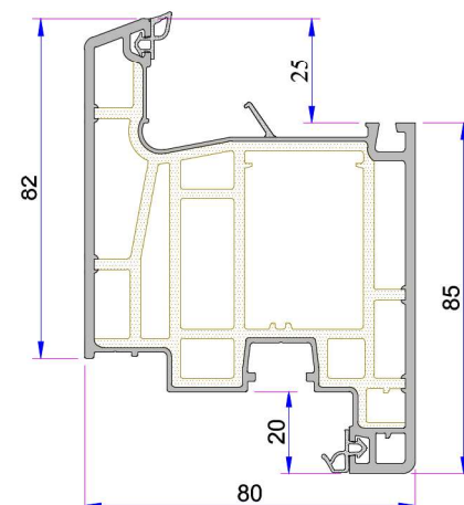
Door Sash Profile P.A.883.2100.600.2.BC.01
