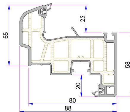
Offset Type Sash Profile P.A.883.2200.600.2.BC.01
