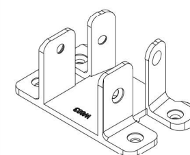
Mullion Connector 21380.0883.0.2
