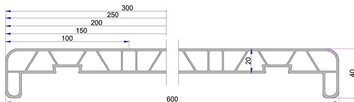
PVC Sill Profile (600mm) P.DNZ.01.60.E.600.19
