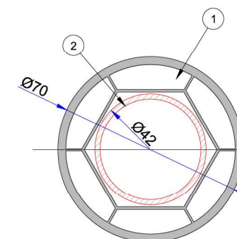
1. Ø70 Pipe Profile P.A.080.5106.600.0.00.19 2. Reinforcement (Ø42) 1,2mm - 34022 - 12502 1,5mm - 34022 - 15502 2 mm - 34022 - 20502
