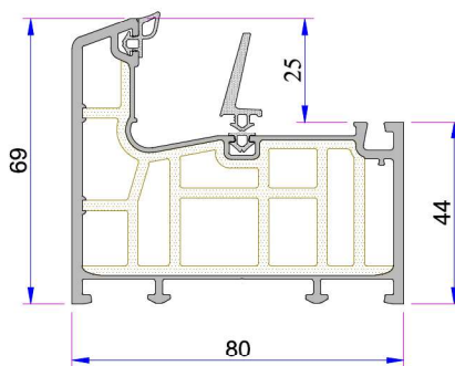
Frame Profile P.A.883.1000.600.2.BC.01
