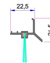
Alm. Threshold Offset Profile (In Process)
