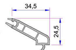
22mm Glazing Bead P.A.433.4000.600.0.HC
