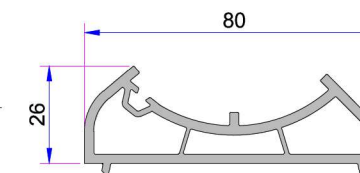
Angled Pipe Adapter Profile P.A.080.5104.600.0.00.19
