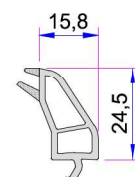
42mm Glazing Bead P.A.777.4302.600.0.HC
