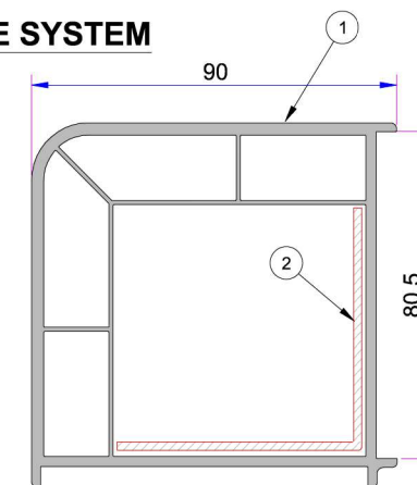
1. 90° Corner Profile P.A.080.5100.600.0.00.19 2. Reinforcement (60x60) 1,2mm - 34022 - 12306 1,5mm - 34022 - 15306 2 mm - 34022 - 20306
