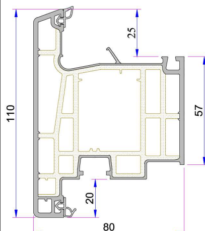
Outward Opening Door Sash Profile P.A.883.2101.600.2.BC.01
