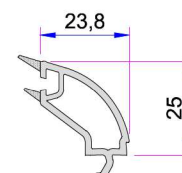
32-34mm Glazing Bead P.A.777.4204.600.0.HC
