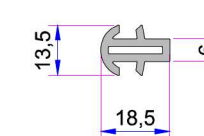
Short Coupling Profile P.A.099.5003.600.0.00.19
