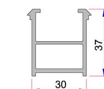
Frame Montage Profile P.A.060.5301.600.0.00.19
