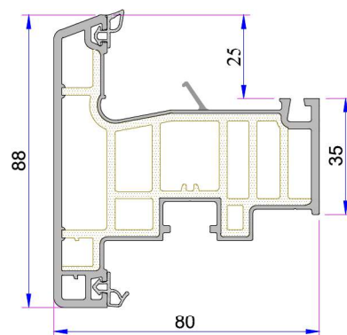
Outward Opening Sash Profile
