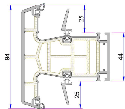
Mullion Profile P.A.883.3000.600.2.BC.01
